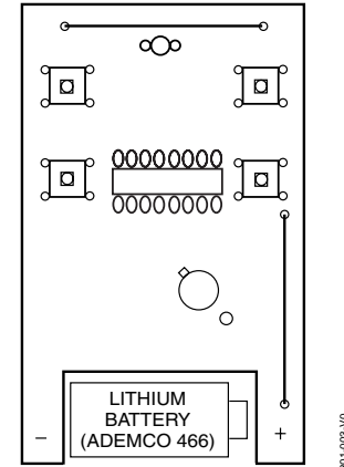
Figure 2. 5801 (Cover Removed)
